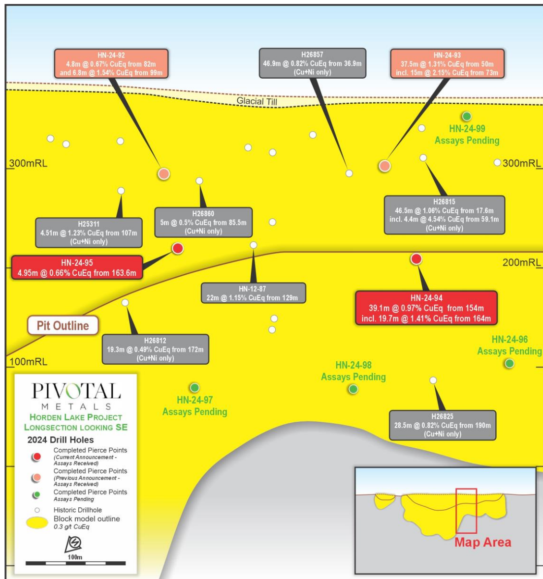
Figure 2: Longitudinal section looking southeast through the Horden Lake deposit
