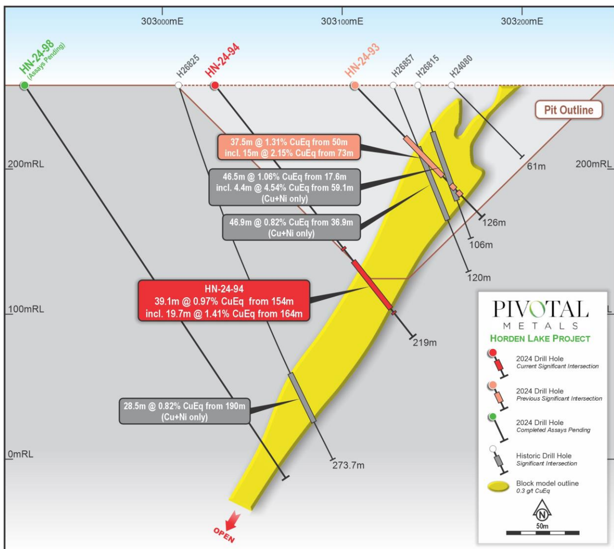
Figure 3: Cross section through HN-24-93 (±30m), Horden Lake deposit
