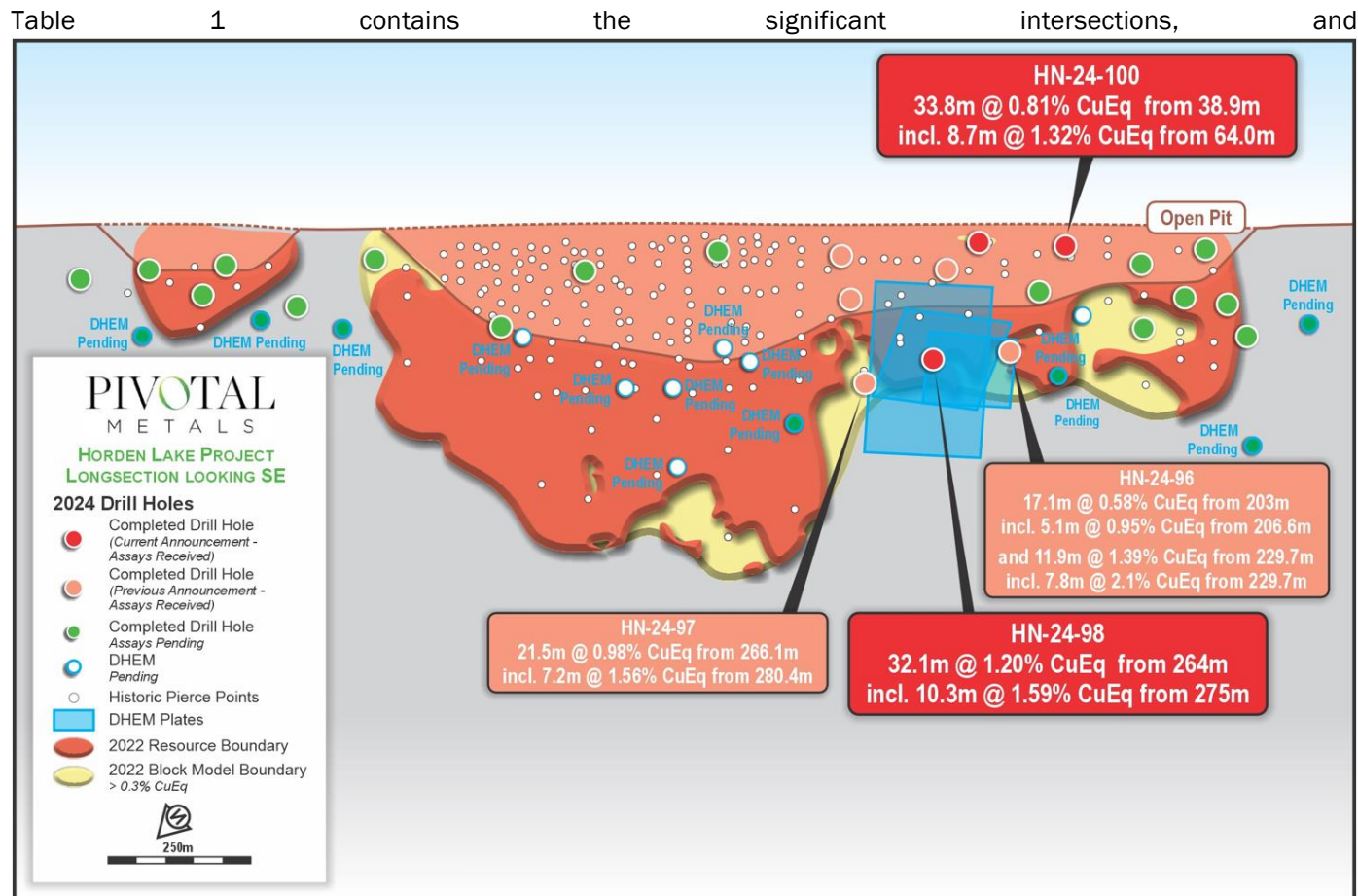
Figure 2 is a longitudinal section showing the spatial distribution of historical and new drill hole pierce points, and DHEM plates associated with the reported survey holes.
