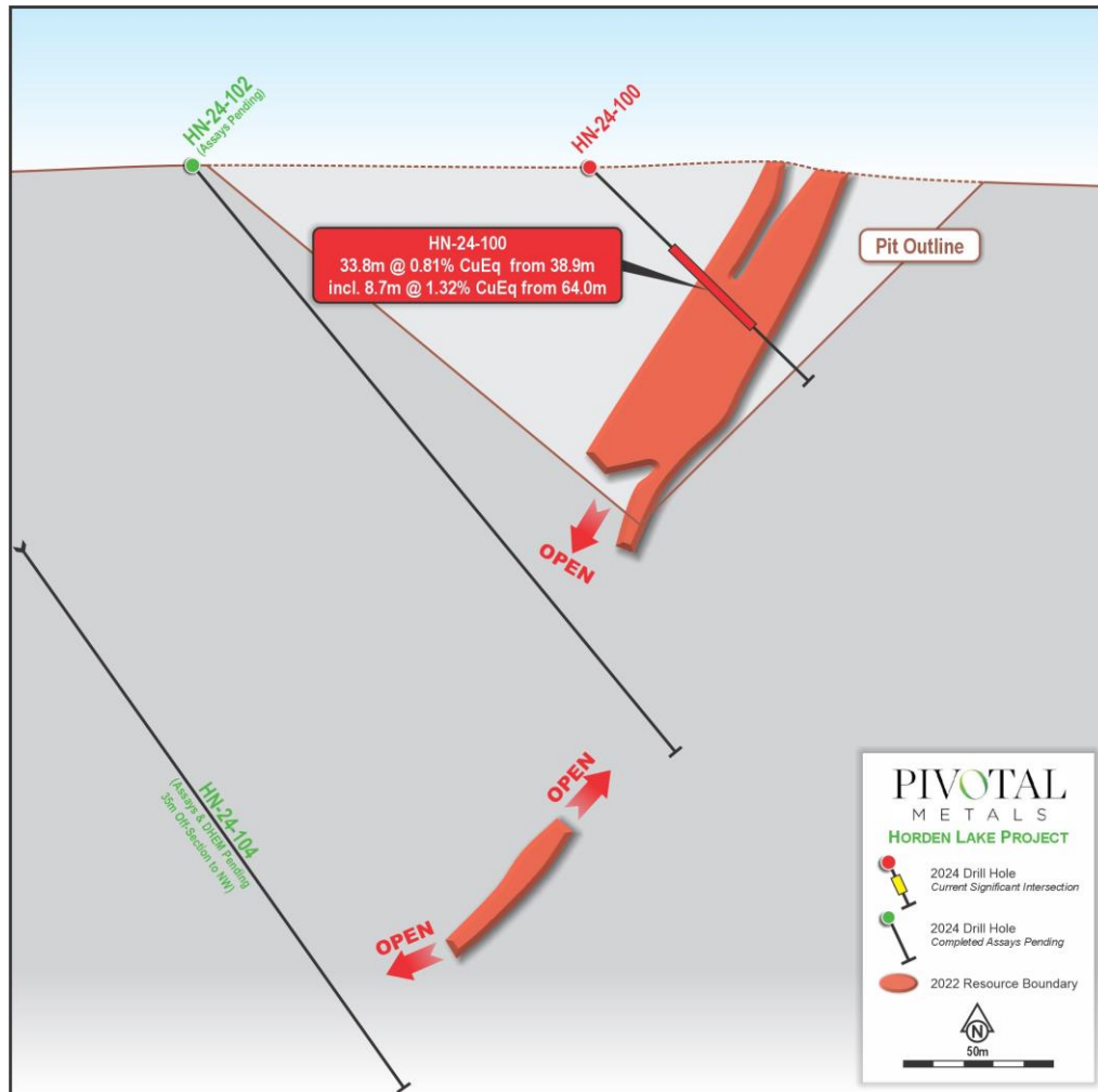
Figure 5: Cross section through HN-24-100 ( \pm 10 m), Horden Lake deposit
