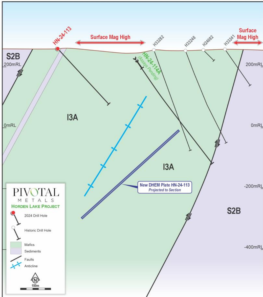
Figure 3: Section through HN-24-113 showing geological units
