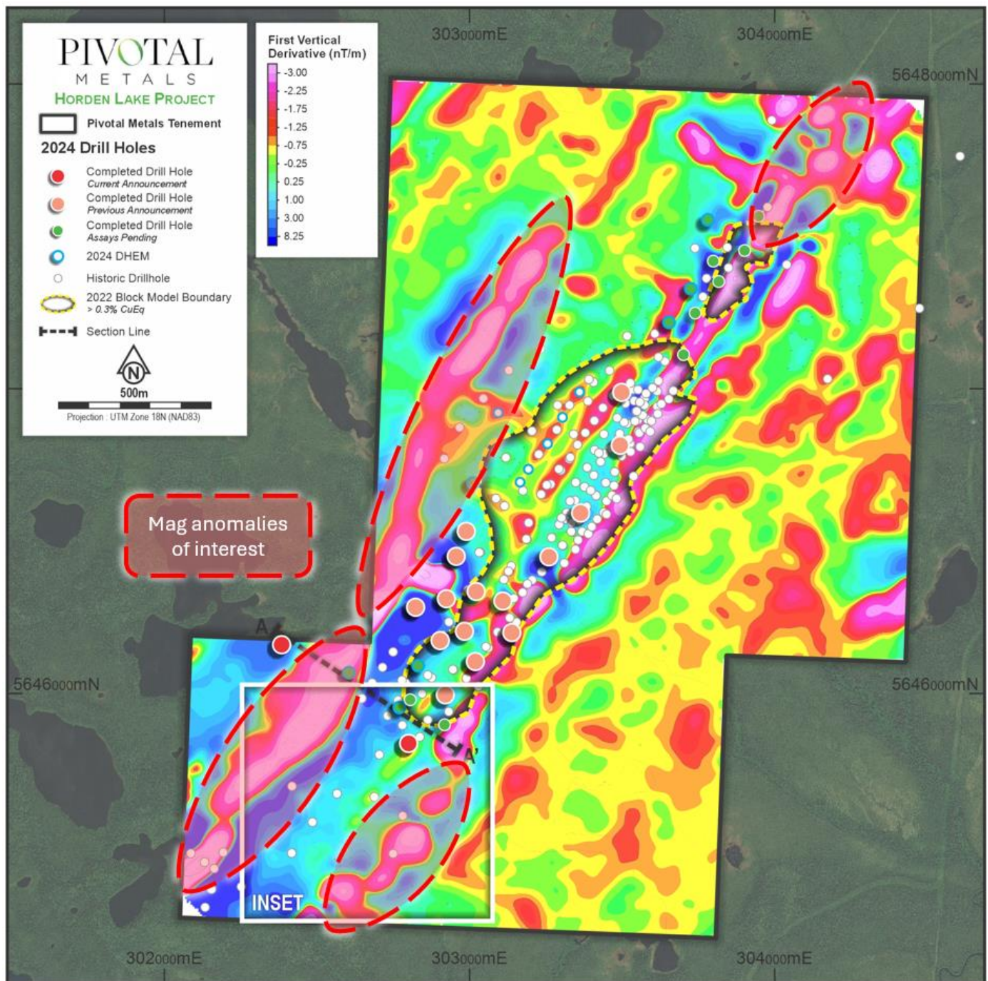
Figure 2: UAV (drone) Magnetic Survey of Horden Lake Project
