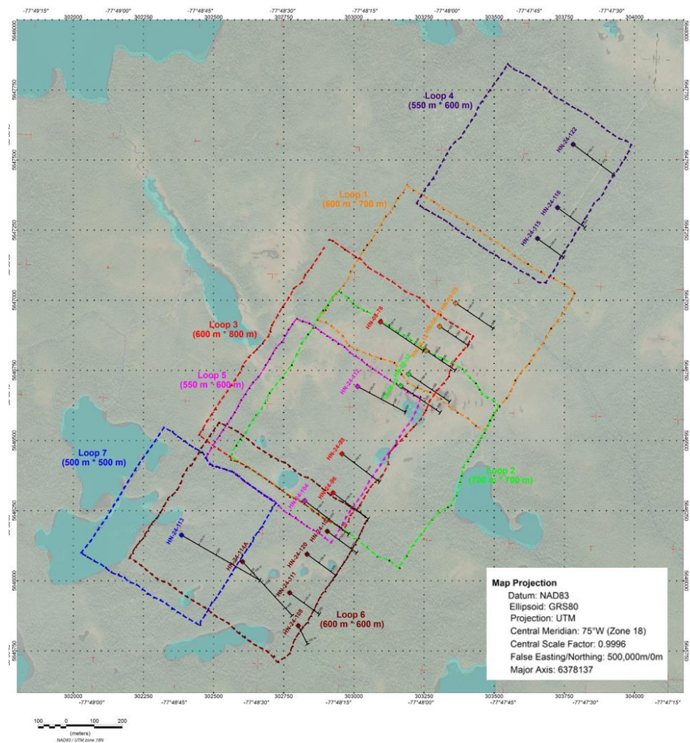
Figure 5: DHEM Loop Locations
