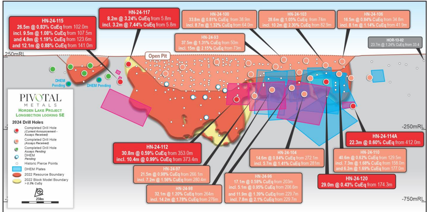
Figure 2: Longitudinal section looking southeast through the Horden Lake deposit
