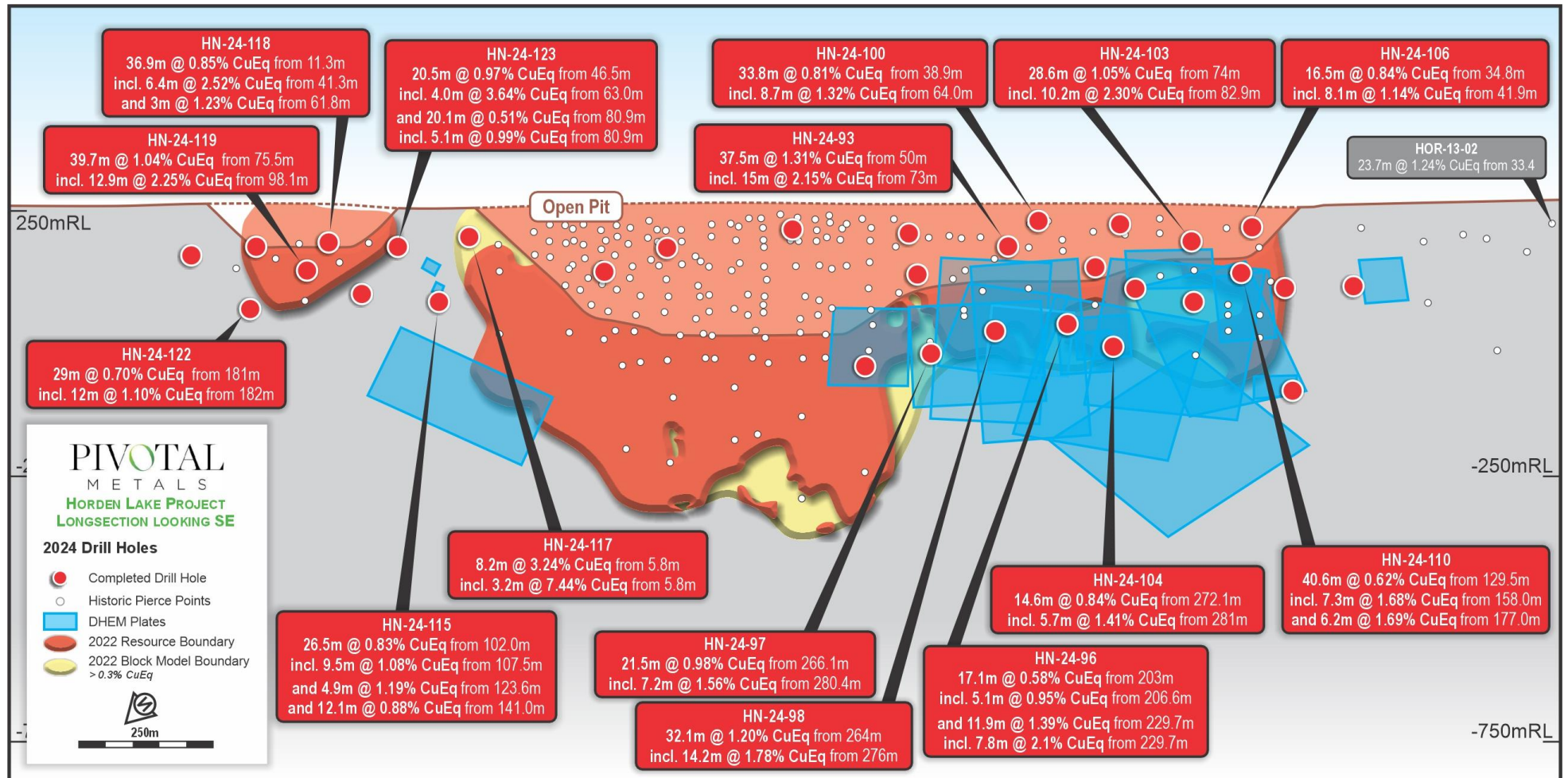
Figure 2: Long section looking SE through the Horden Lake deposit, showing selected highlight intercepts, the DHEM modelled conductor plates interpreted to represent the potential continuation of the Horden Lake sulphide mineralisation
