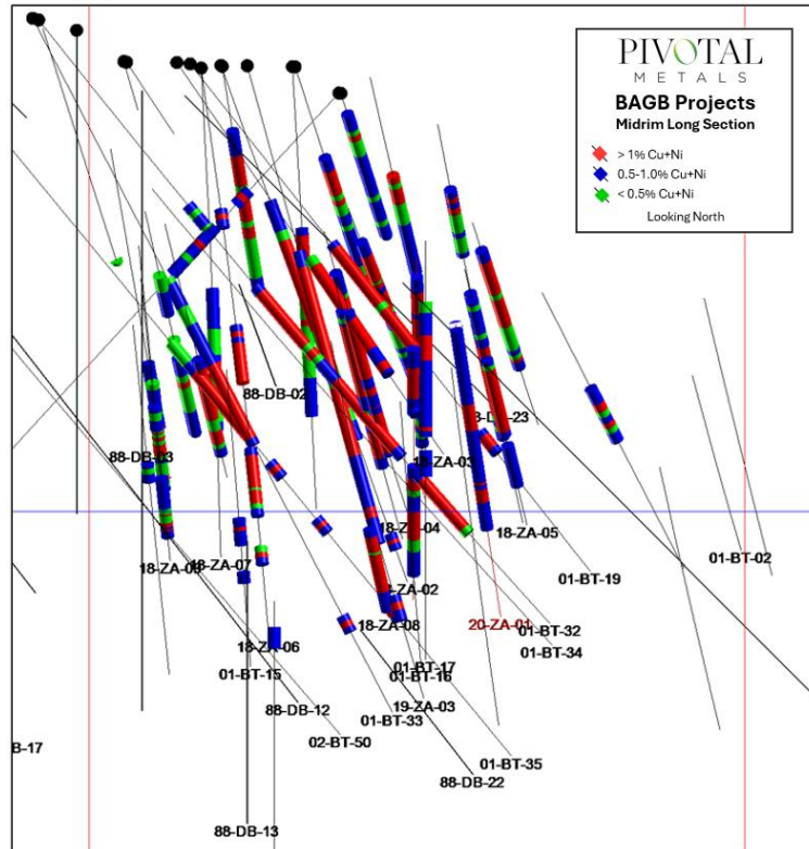
Figure 6: Midrim occurrence long section A-A', illustrative of the described high-grade accumulations "trapped" in pockets at the known occurrences
