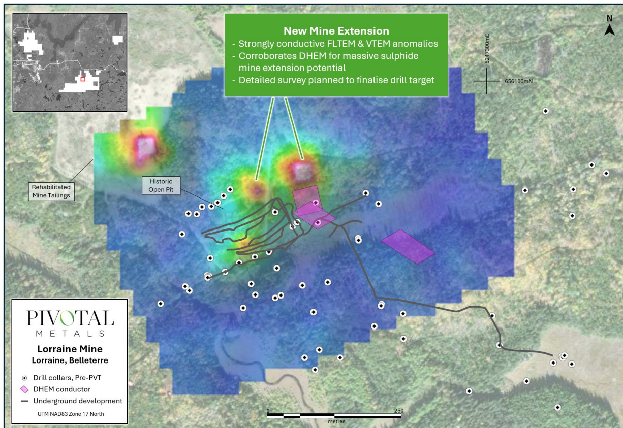
Figure 2: Lorraine Mine Cu-Ni-Au extensions, showing FLTEM total field intensity (channel 15)
