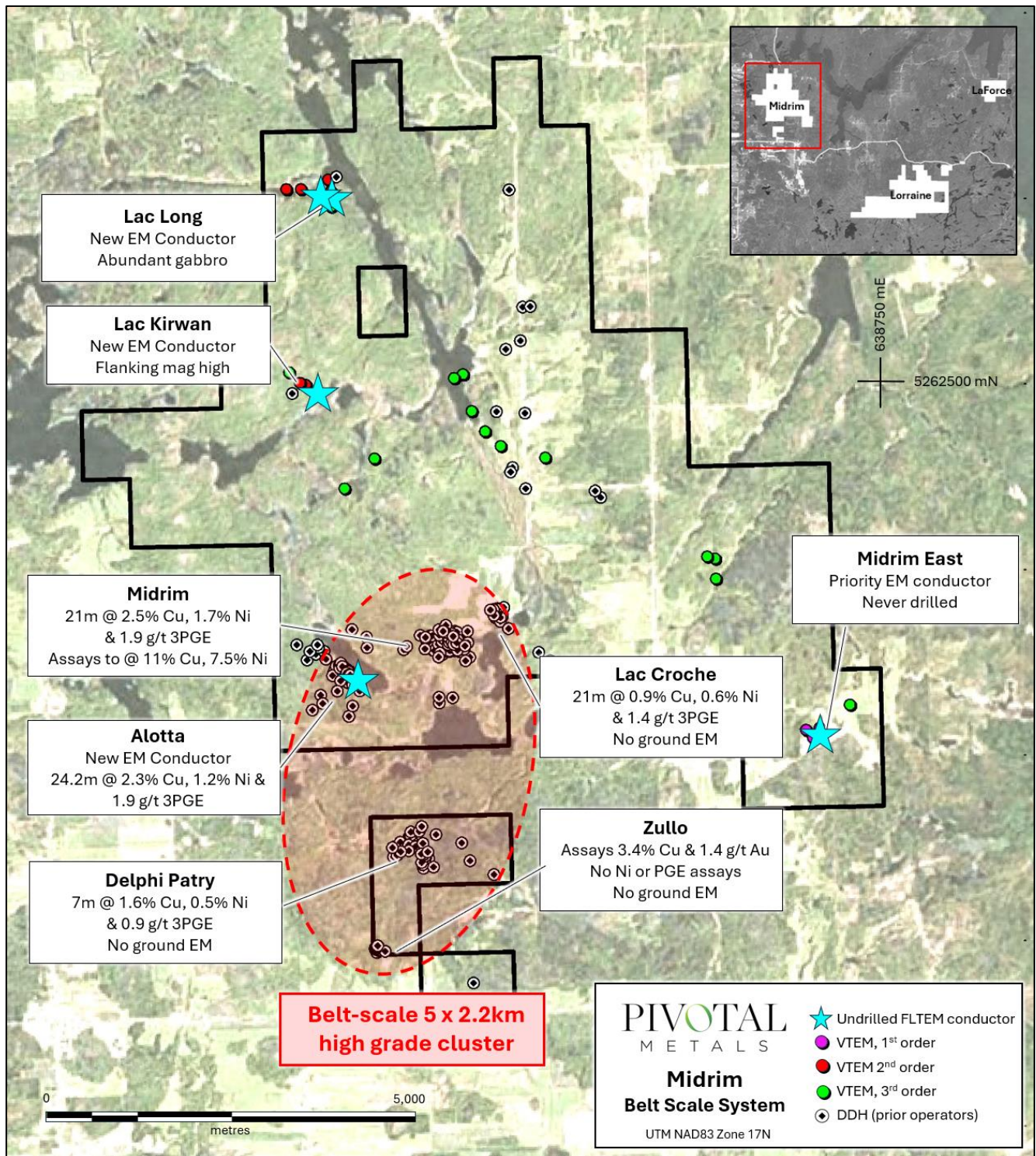
Figure 4: Midrim project area showing widespread high grade mineral occurrences and geophysical anomalism, and limited drilling outside of the historical target areas
