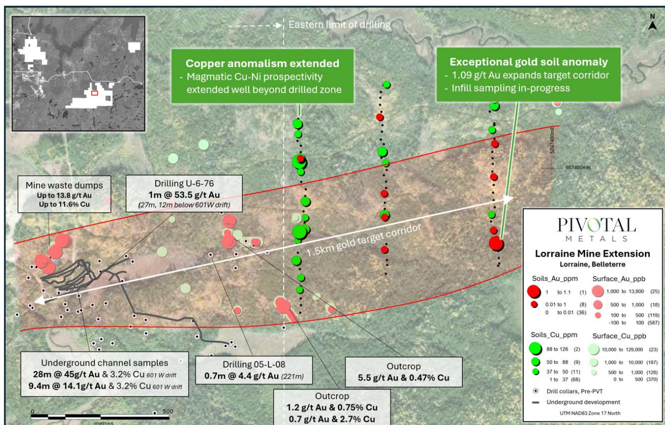
Figure 5: Lorraine Mine gold high-grade gold target.
