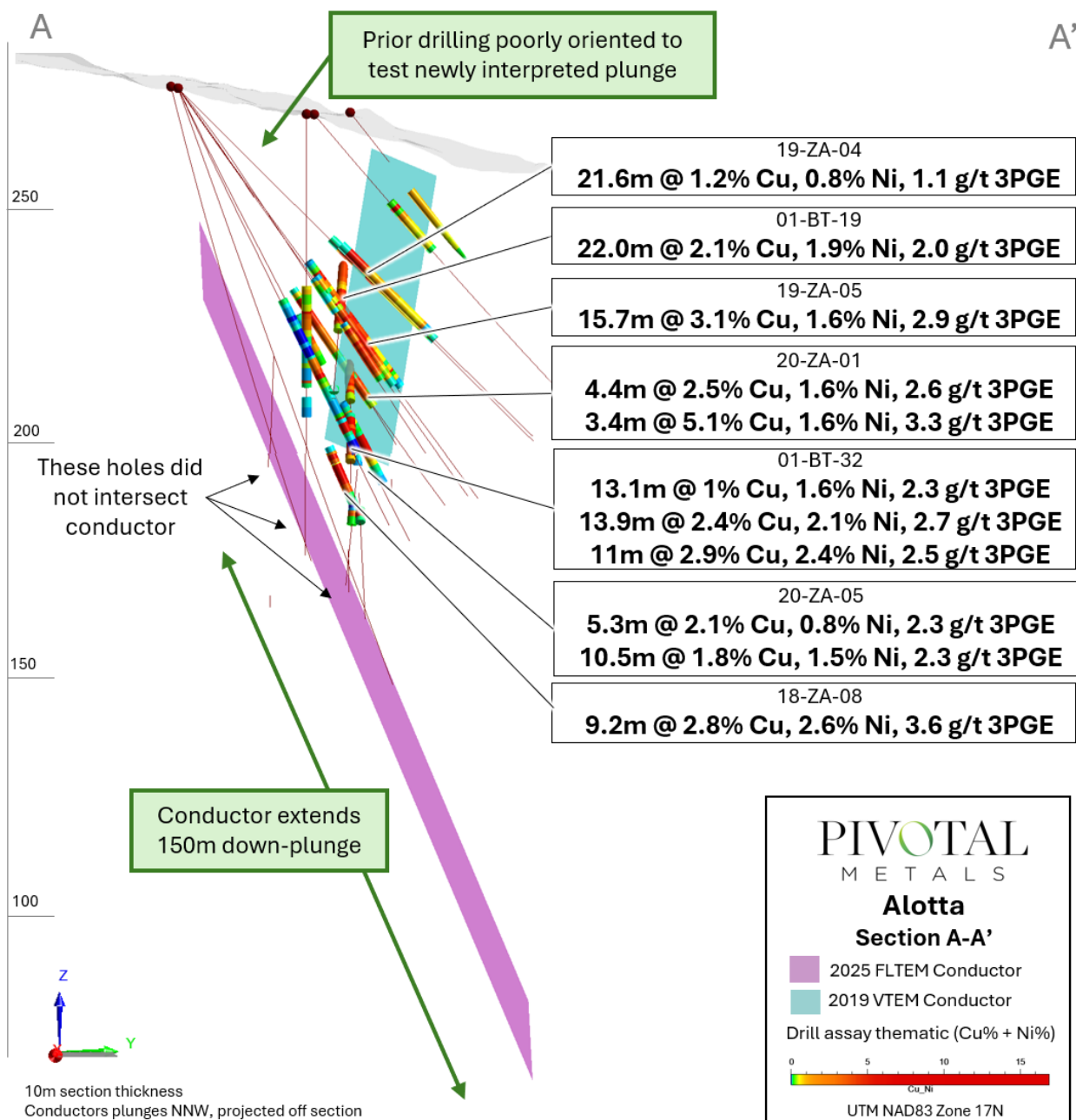
Figure 3: Section view of Alotta showing high-grade mineralisation and interpreted FLTEM conductor extending strongly down-plunge. Note orientation of prior drilling poorly oriented to intersect newly interpreted plunge.
