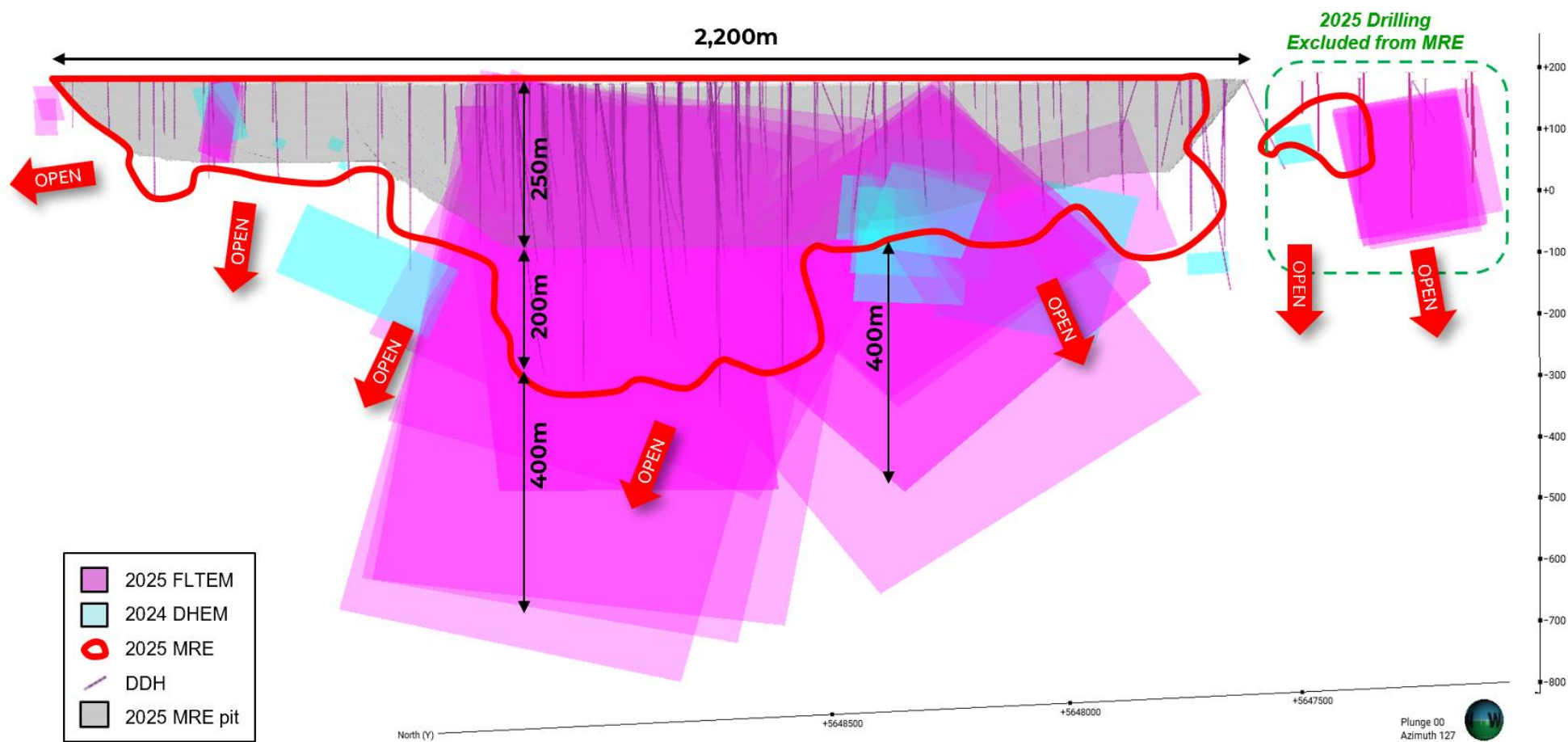
Figure 6: Long section looking SE outlining the 2025 Horden Lake MRE superimposed onto the modelled conductor plates interpreted to represent the potential continuation of the Horden Lake sulphide mineralisation.
