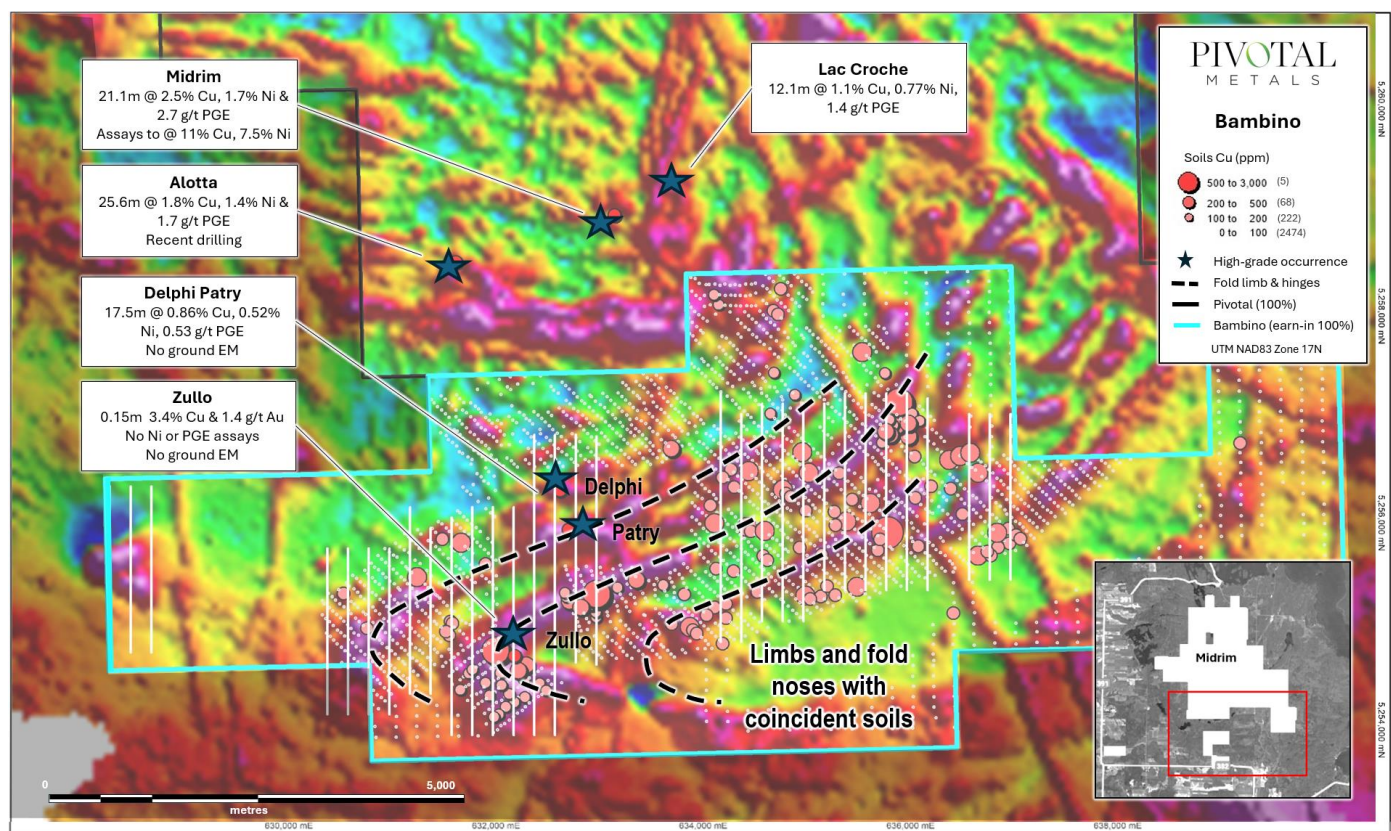
Figure 3: Bambino prospective horizon, and planned IP survey lines in white
