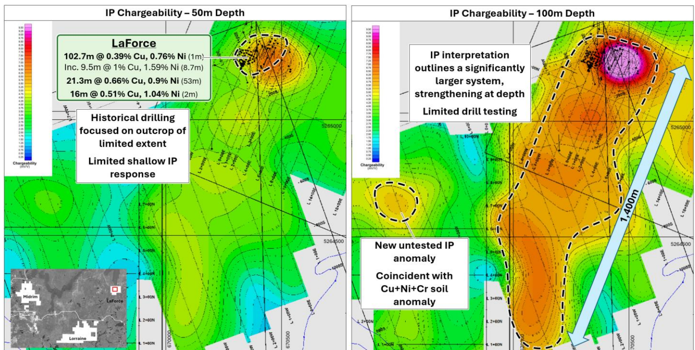
Figure 1: LaForce merged historic IP interpretation at 50m and 100m, showing the 1.4km newly defined depth trend extending from the known Cu-Ni occurrence
