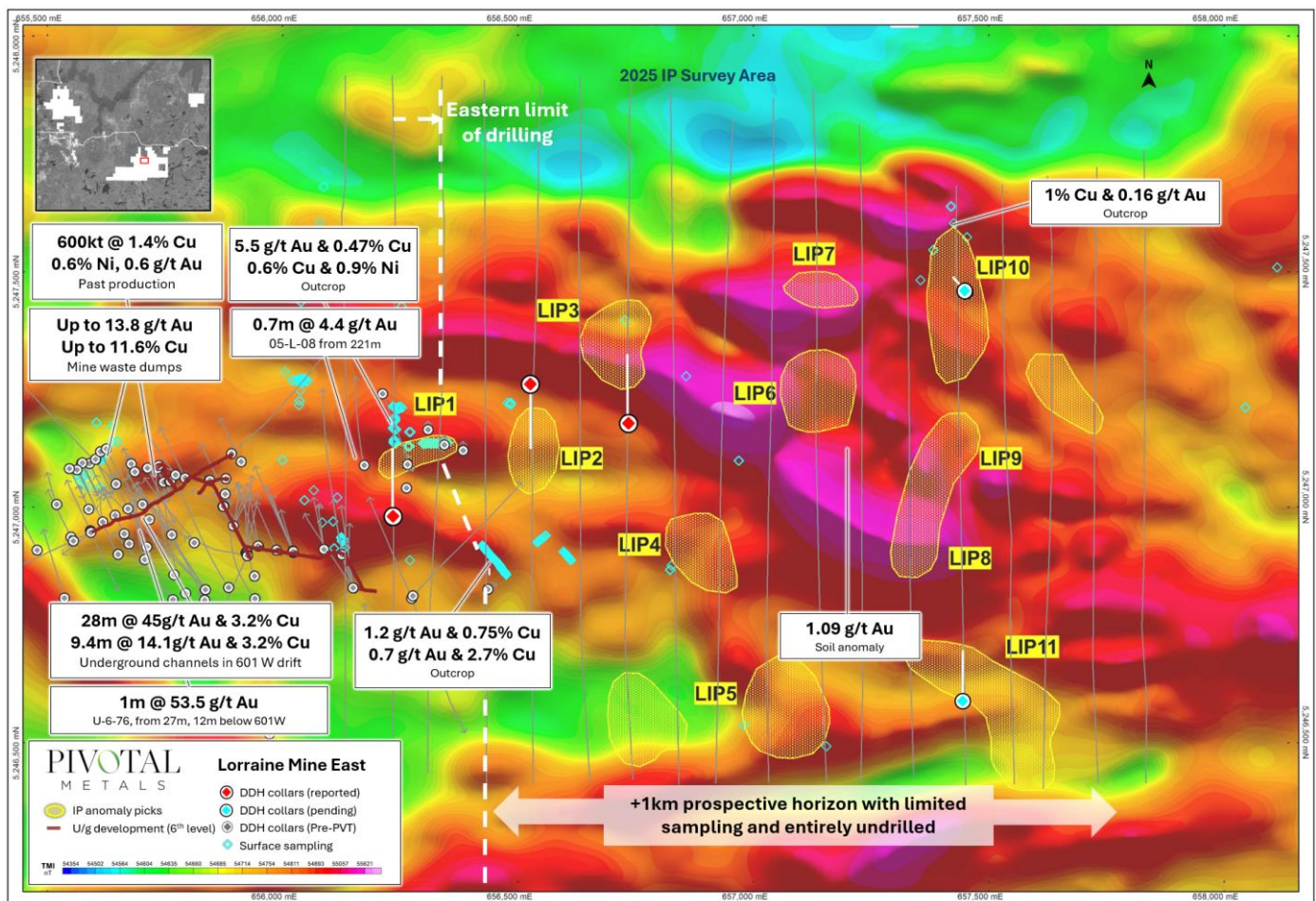
Figure 2: Lorraine Mine East IP targets and 2026 drill collar locations
